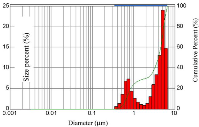
Fig. 8. Dynamic light scattering size distributions of individual tubes and the agglomerates of smaller sizes for the fine-agglomerates of MWCNTs.
